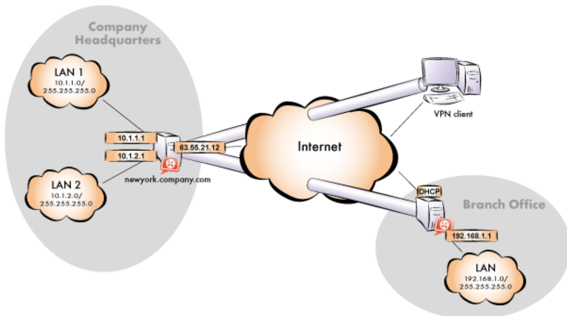
Figure 23.12 Example — interconnection of the headquarter and a filial office by VPN tunnel (connection of VPN clients is possible)
