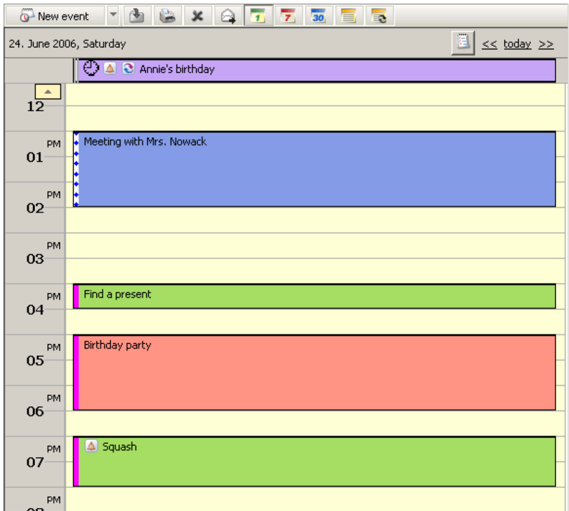
Figure 1.65 Day view
