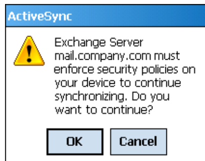
Figure 4.37 Wipe confirmation
