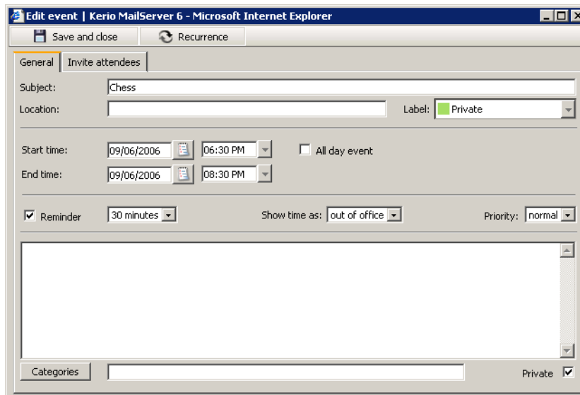
Figure 1.124 Event settings
