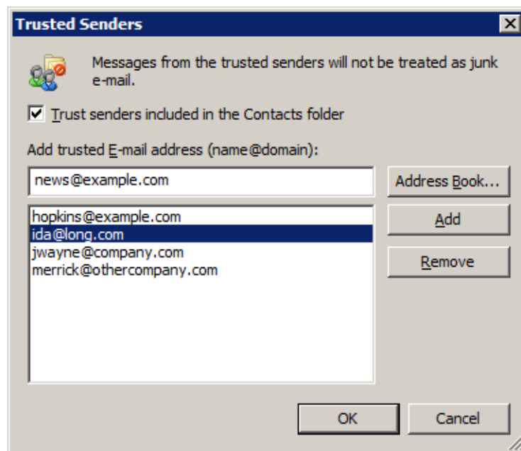
Figure 6.23 Trusted Senders
