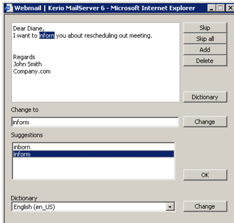
Figure 1.36 Spellchecker
