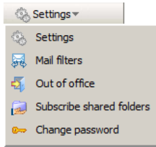
Figure 1.113 Settings Menu
