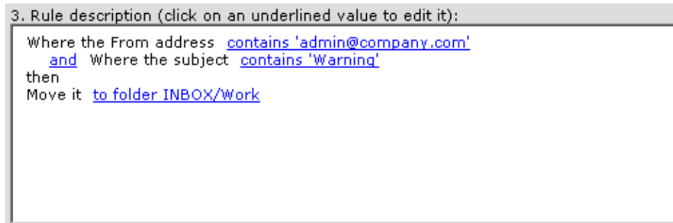
Figure 1.133 Rule Description
