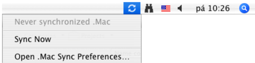
Figure 12.8 Starting synchronization
