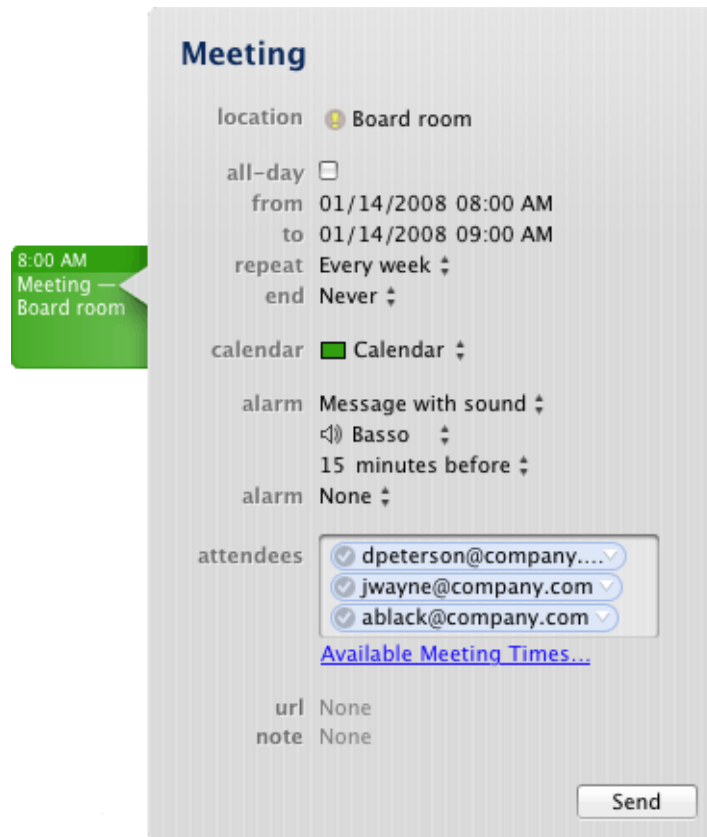
Figure 11.10 Meeting settings
