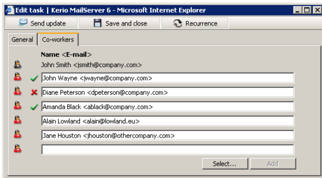
Figure 1.85 Task acceptance/rejection
