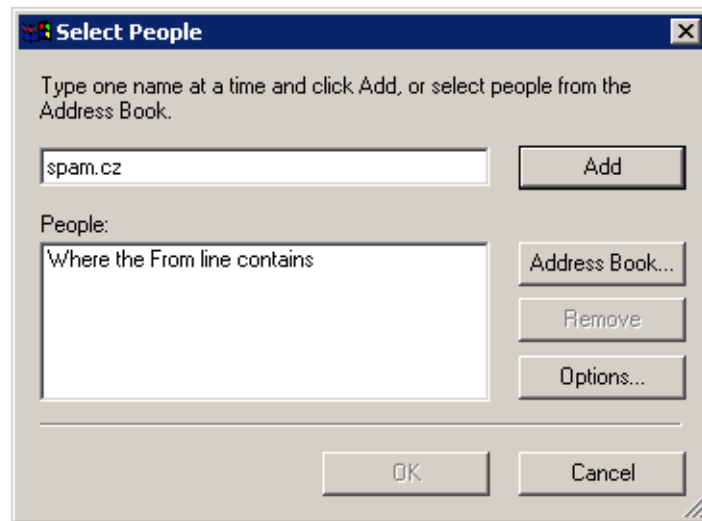
Figure 6.19 Select People
