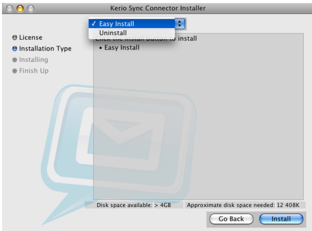
Figure 13.2 Installation settings
