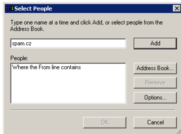
Figure 5.21 Select People
