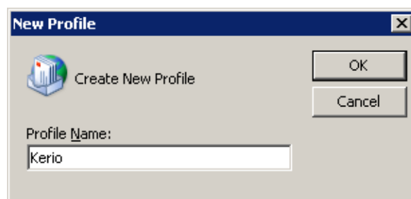
Figure 5.3 New profile
