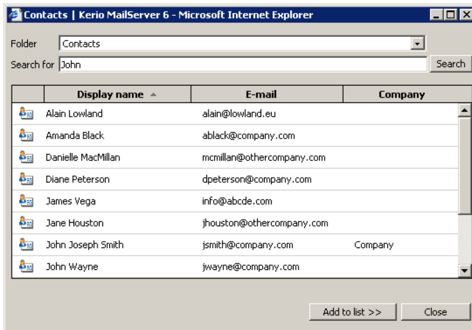
Figure 1.59 Select
