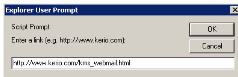
Figure 1.34 Link
