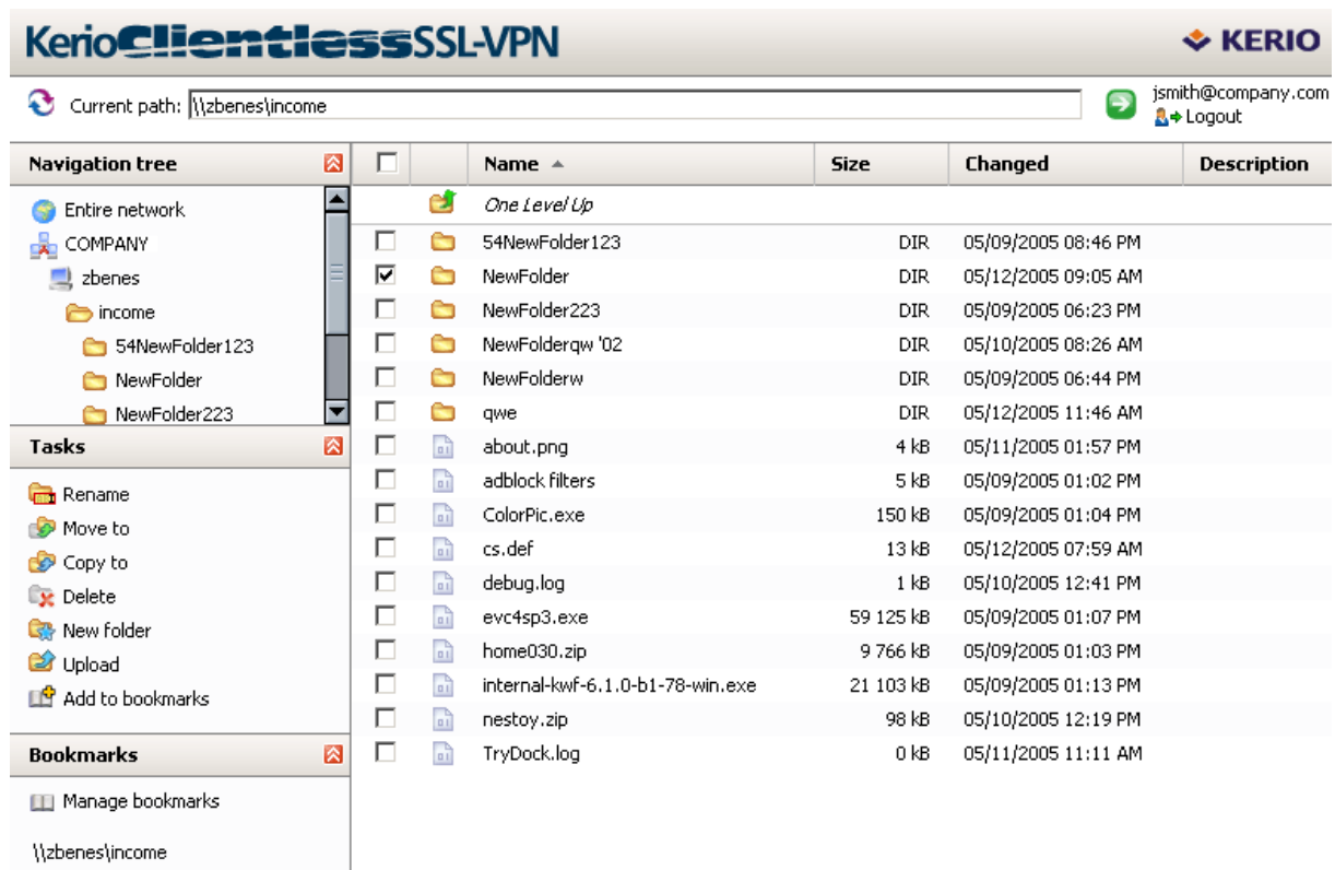
Figure 4.2 Clientless SSL-VPN — main page
